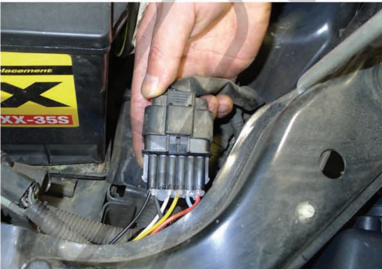
33. Connect the headlight harness to the projector headlight Please see the "L. E. D. head lights installation instructions"
