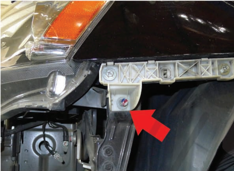
25. The 10mm bolt location
