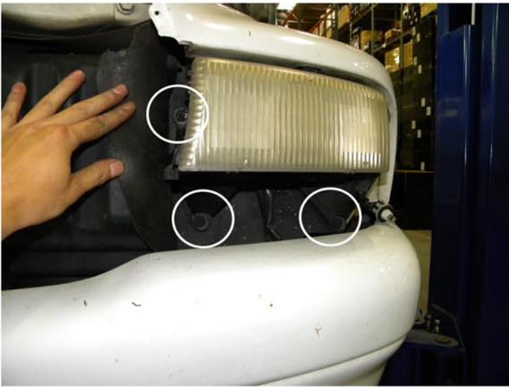
5. Remove three 10mm headlight bolts
