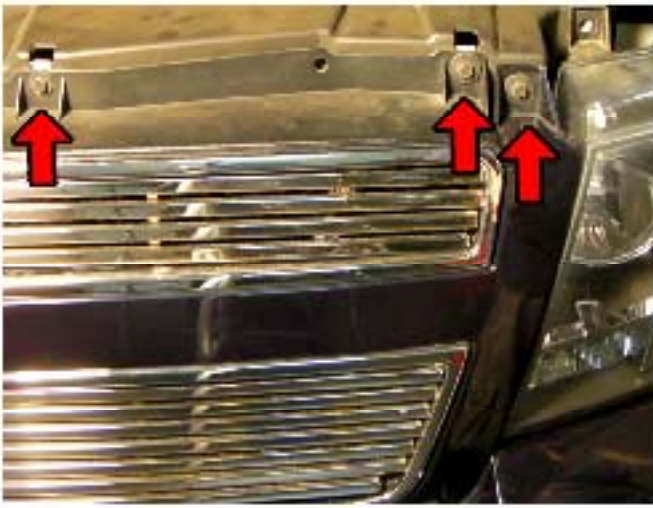
17. Install three screws from the top of the grill
