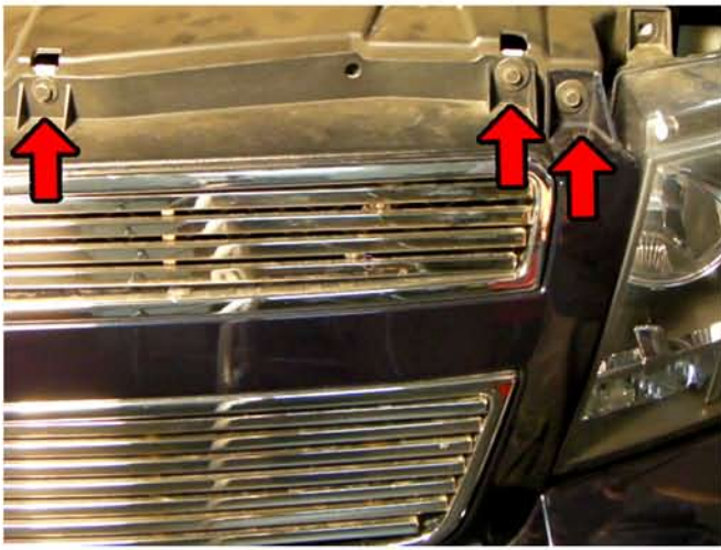
5. There are three bolts need to remove on the grill
