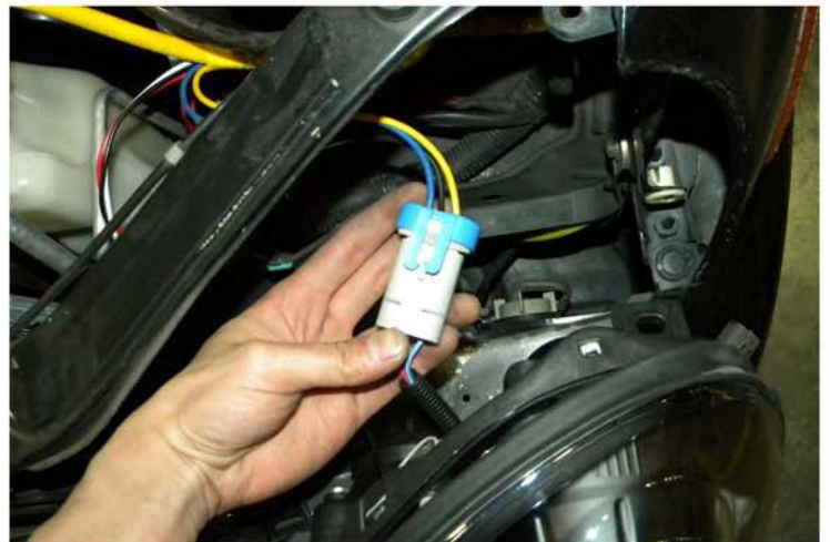
16. Connect the headlight harness to the new headlight
