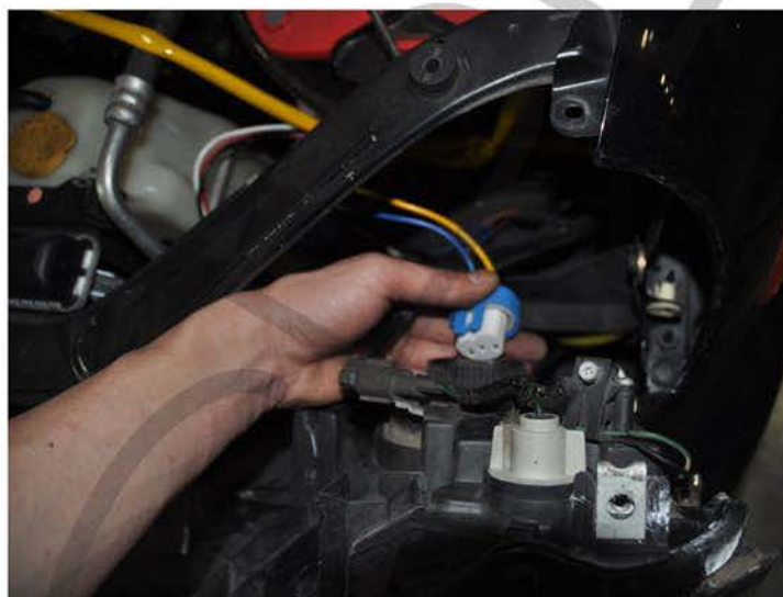
9. Disconnect the headlight harness
