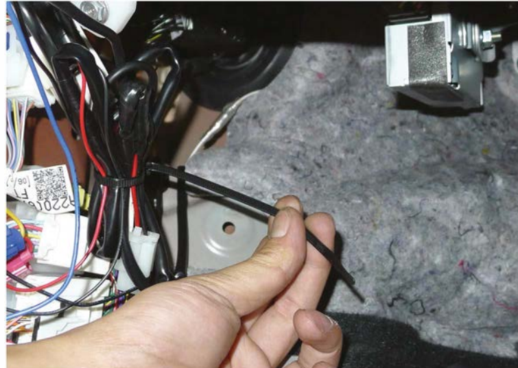
52. Zip tie loose wiring to the factory harness
