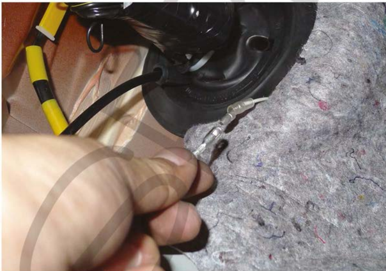
51. Connect the switch harness to the fog light harness
