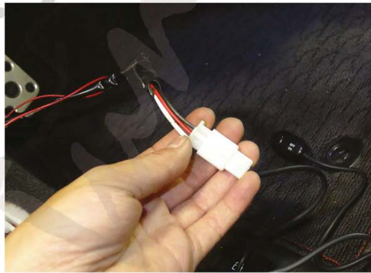
32. Connect the switch to switch harness
