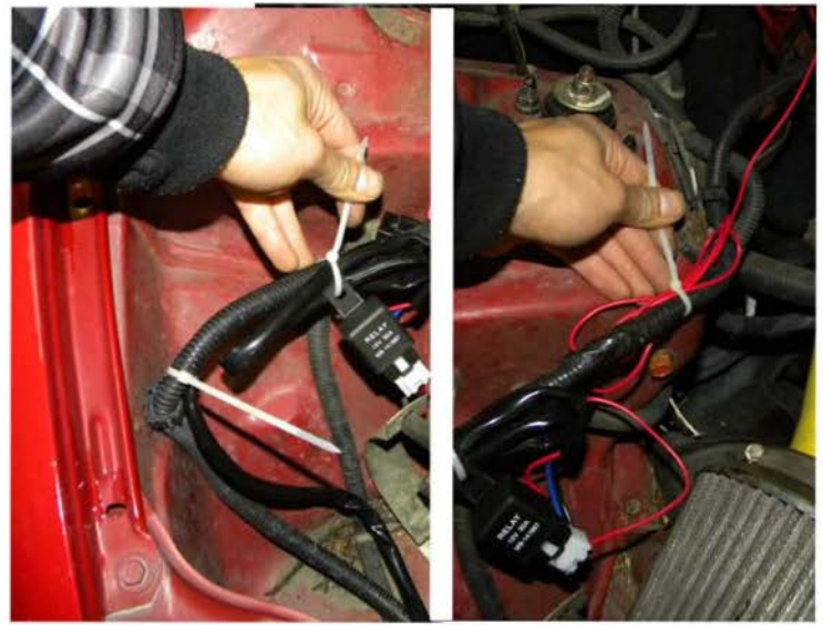
30. Zip the excess wiring and relay to the stock harness
