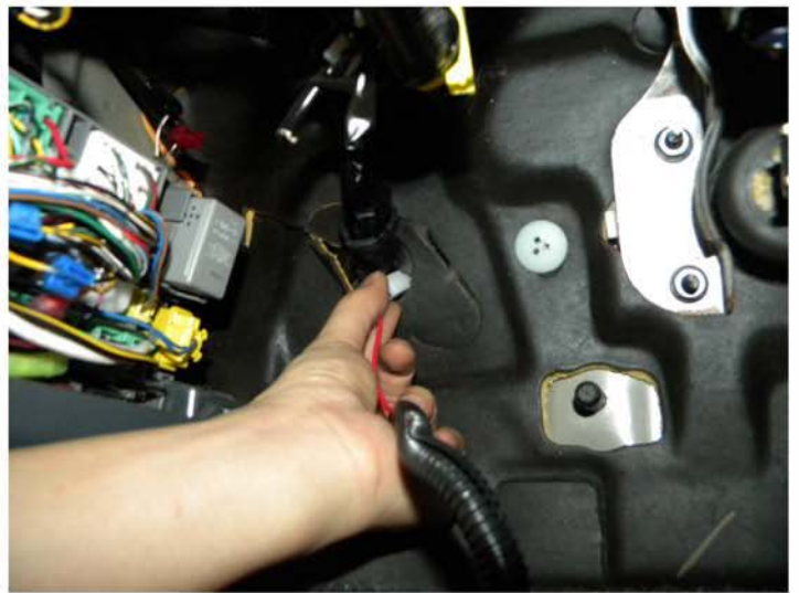
34. Run the switch power wire through the rubber grommet
