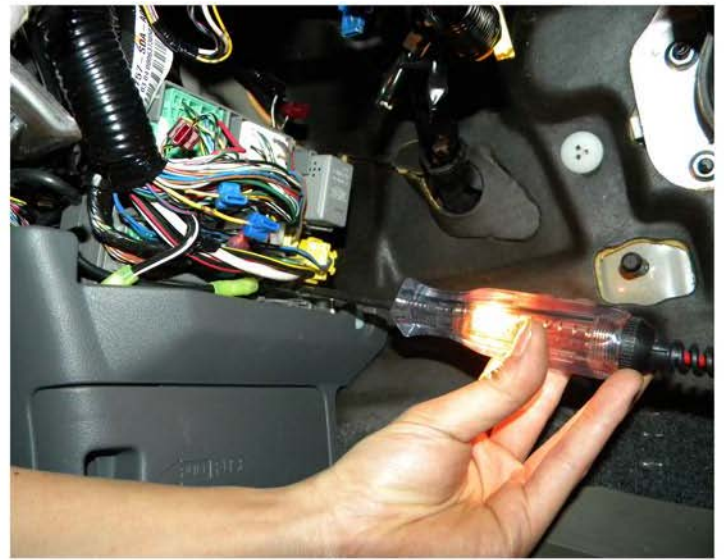
30. Use the test light to locate the battery power line and the ACC power line
