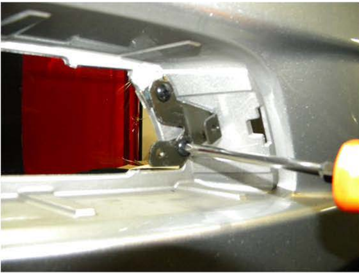
17. Secure mounting bracket with (2) phillips head screws
