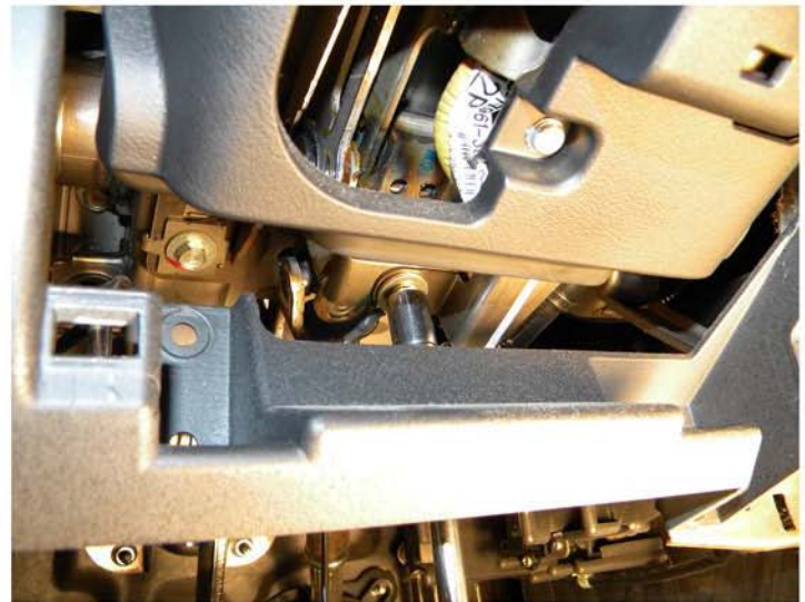
32. Secure the switch harness ground wire with the 10mm bolt
