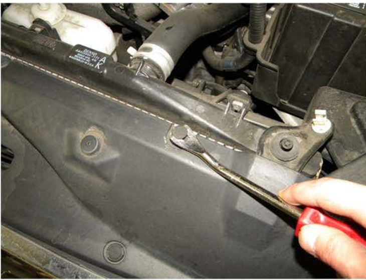
5. Remove the (10) plastic clips
