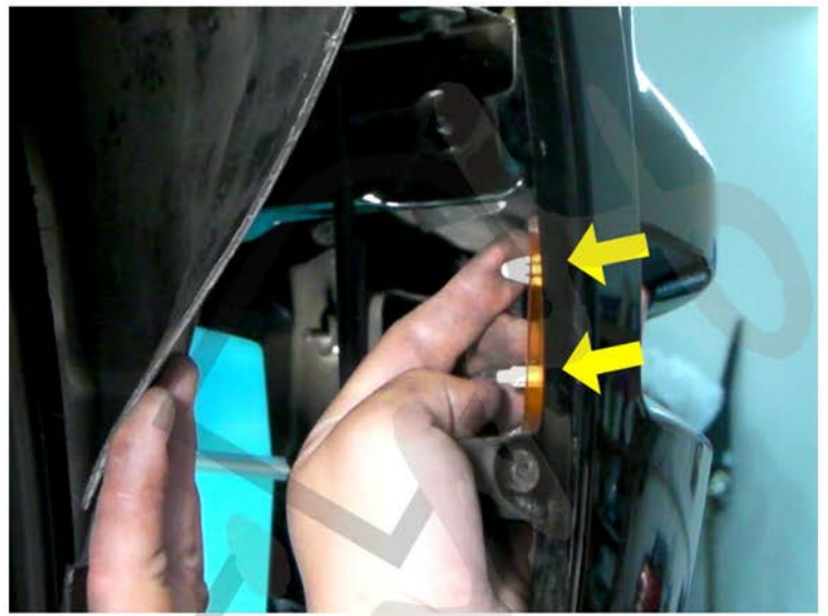
6. Squeeze two clips to remove the bumper light
