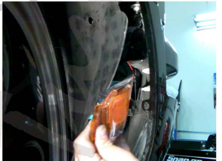
8. Remove bumper light
