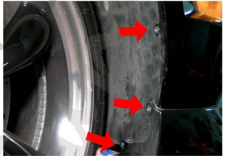
2. Remove three bolts under wheel well
