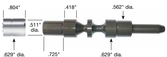
Pressure Regulator Valves and Sleeves Cannot Be Interchanged
