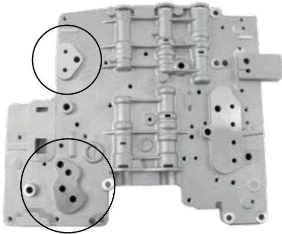
Different Sized Pressure Regulator Valves and Sleeves
