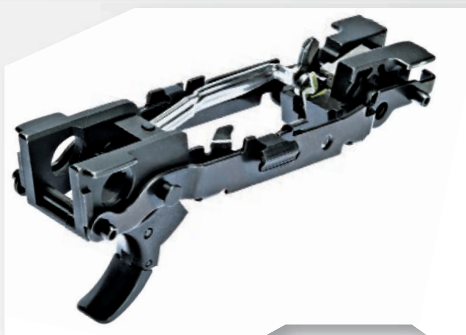
STAINLESS STEEL CHASSIS STEEL-TO-STEEL CONNECTED SYSTEM
