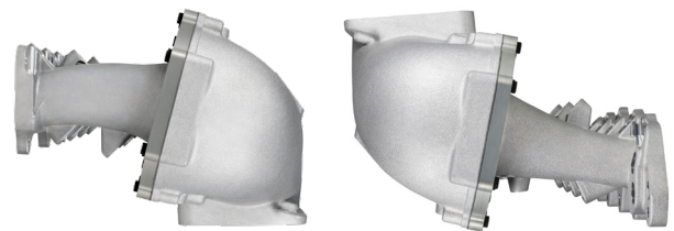
Centerfeed manifold is available in the K-Series (left) and B-Series (right) applications.
