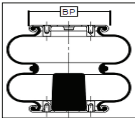
Double Convoluted
