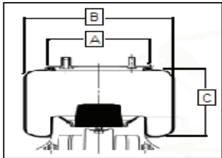
Rolling Lobe
