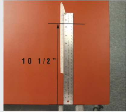
Measure from the front deck lid edge rearward 10 1/2"
