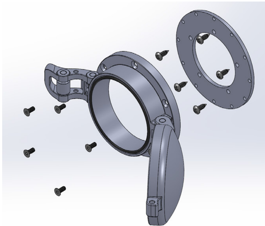
CSX-9030-A (exploded view)
