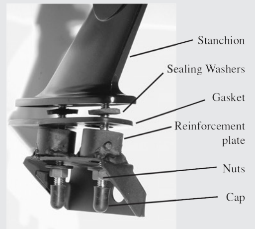
Wing mounting hardware
