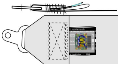
example of a left shoulder belt with FIA main and hologram label, which must always be sewn together
