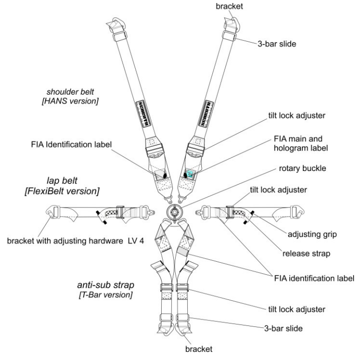
drawing shows standard Profi II-6H racing harness
