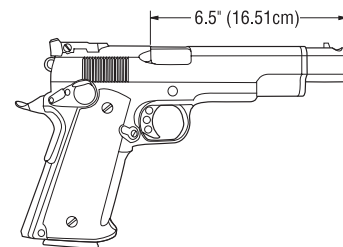
Competition pistol barrel lengths are measured from the back portion of the ejection port to the end of the compensator.
