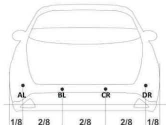
For Rear: 4 sensors installation
