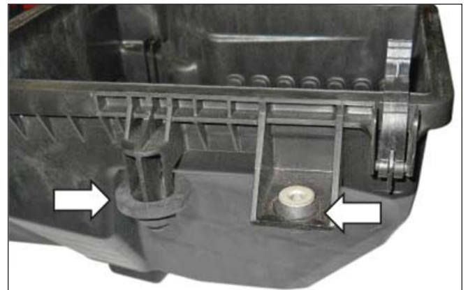
16. Remove the rubber isolator from the bottom of the stock air box tray and retain for use during installation.
