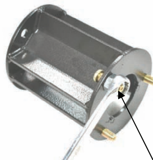
Install studs in strut spacer.
