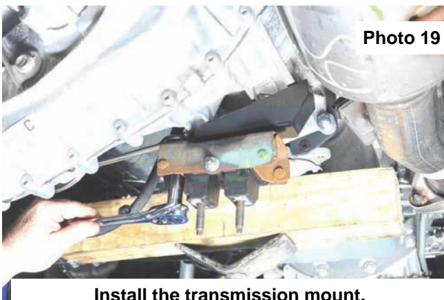
Install the transmission mount.
