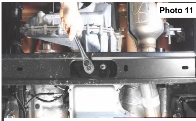
Remove the crossmember from the trans.
