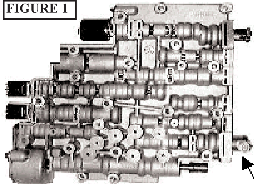
3/2 Downshift Solenoid
