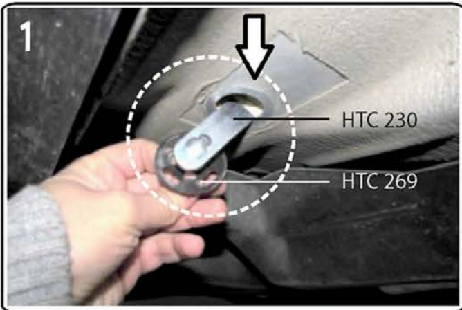
1) Locate rear bracket mounting point insert HTC 230 with HTC 269
