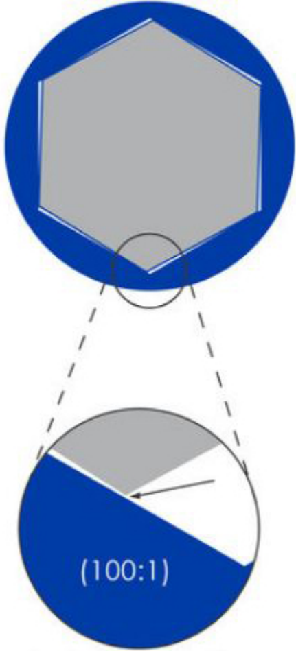
Contact area inside of a socket - 0.3mm
