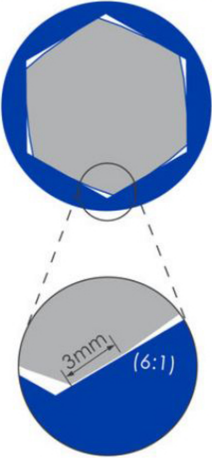
Contact area inside of a socket - 3mm
