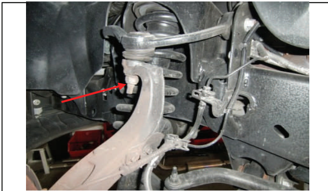
Loosen but do not remove upper ball joint nut
