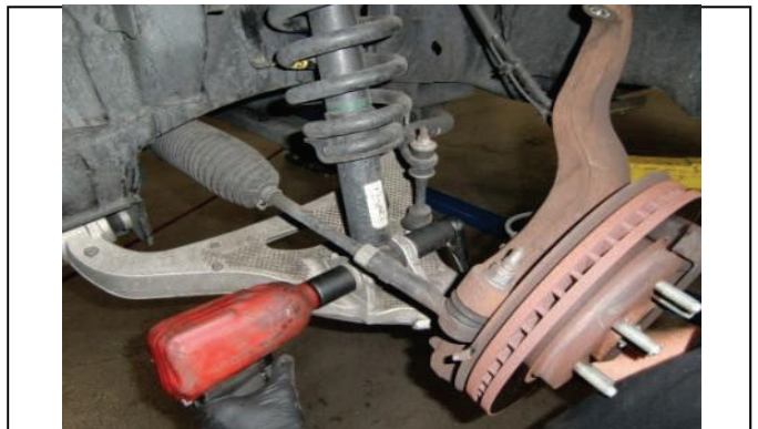
Remove lower strut mounting hardware
