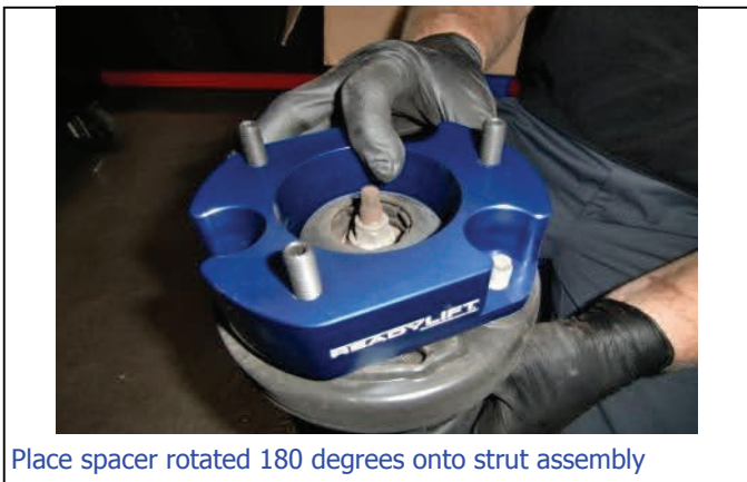
The next (4) steps are for the T6 Billet spacers install only..
