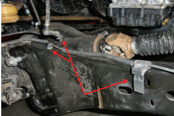
Remove all wiring clips from radius arms
