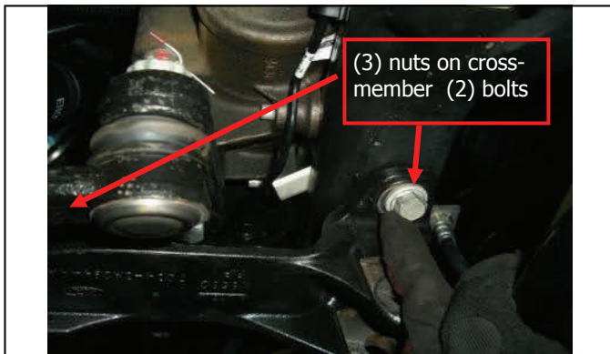
Optional trac bar bracket; Remove mounting hardware (5)
