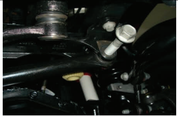
Remove upper trac bar hardware and disconnect at frame.
