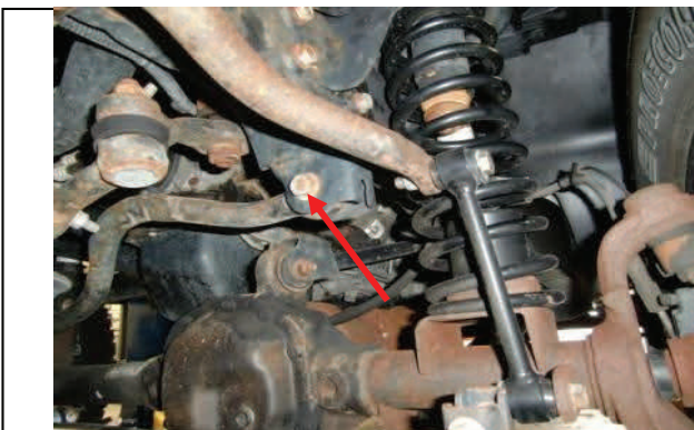
Reconnect front upper trac bar with OE hardware and torque.
