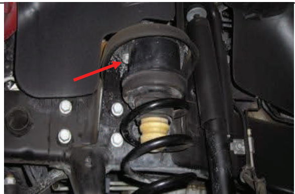
Bolt-in spacers, install OE isolator, then bumpstops & springs
