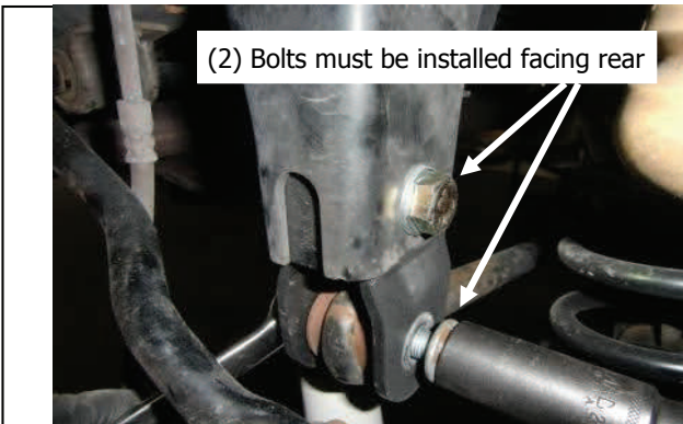
Carefully raise rear axle to reinstall OE upper trac bar bolt
