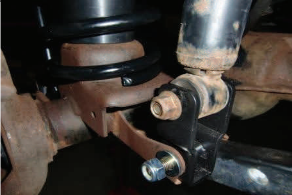
Raise axle and reinstall OE front shocks and torque to spec.
