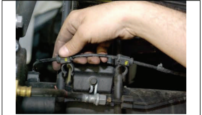
Vehicles with ABS/TC remove clips from U-bolts.
