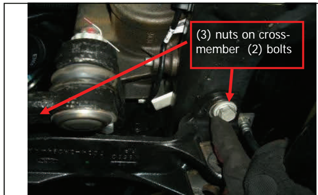
(3) nuts on cross-member (2) bolts Optional trac bar bracket; Remove mounting hardware (5)
