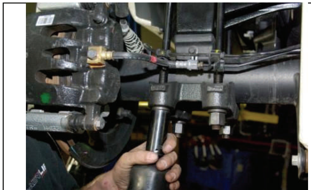
Install longer U-bolts and nuts onto axle plate. Torque later.
