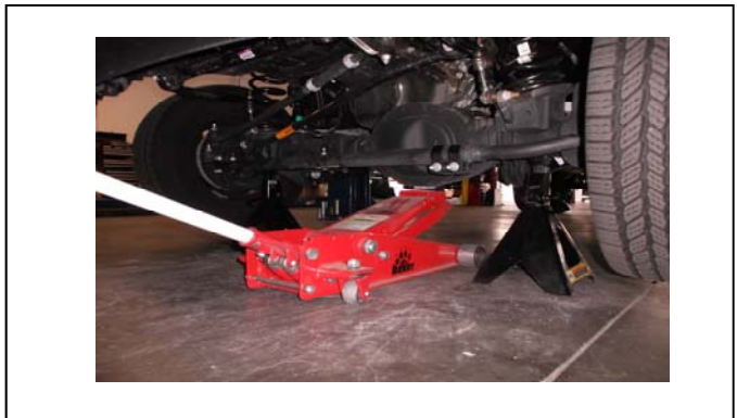
2. Lift the front of vehicle by the frame, then support the axle.
