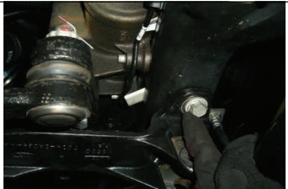
Remove (2) mounting bolts at frame
