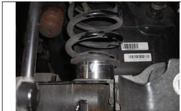
Reinstall coil spring and seat on top of spacer, raise axle.
