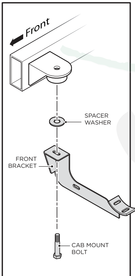
Front Bracket
