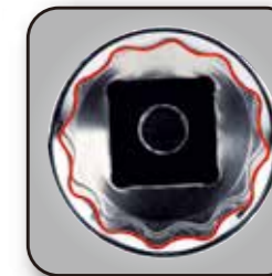
Z-Drive
