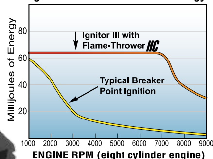
Ignitor III vs. Breaker Point Energy
