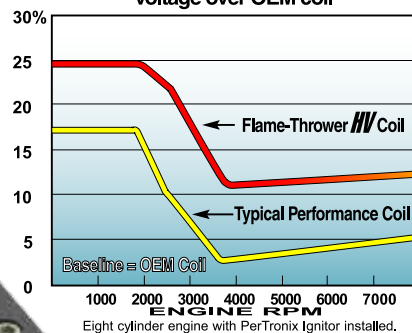
Percent of extra available voltage over OEM coil
