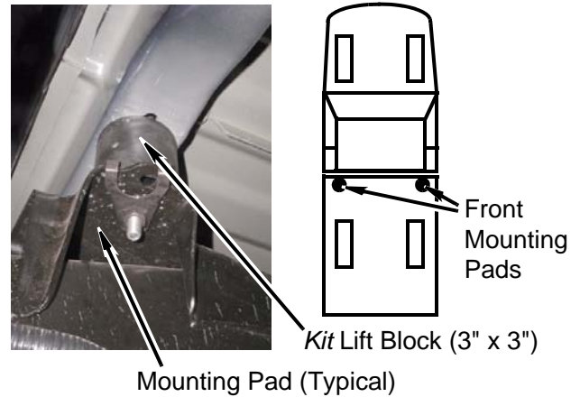
Cab Mounting Locations
