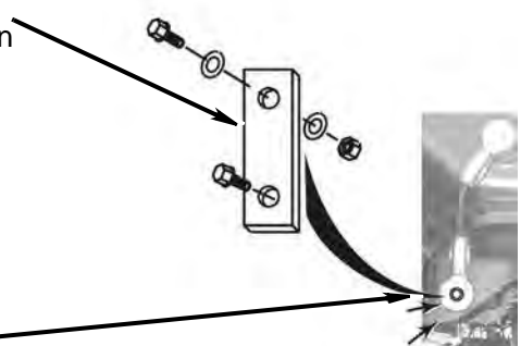
Frame Rear Mounting Pad
