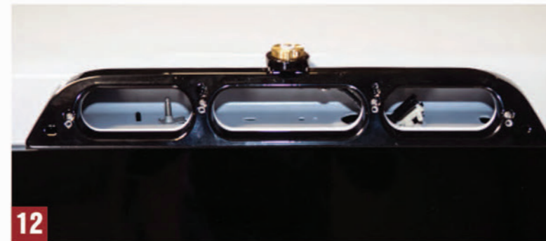
Fig. 8 Route the antenna cable into the cab - follow the brake light harness. From inside the cab, access the cable and route to final desired location. Fig. 9-12 To attach the antenna adapter, align and attach the adapter utilizing the four (4) factory mounting holes and the provided phillips pan head screws. Fig. 13-15 Keep the adapter secured in place. Using the adapter's two (2) top center holes as a guide, drill through the truck body with a 3/16" bit. Next, feed the support bracket through the middle hole of the adapter. Slide the support bracket behind the adapter and the truck body then, match up the support bracket's holes with the ones you just drilled. Use the provided socket head cap screws to secure the support bracket in place.
