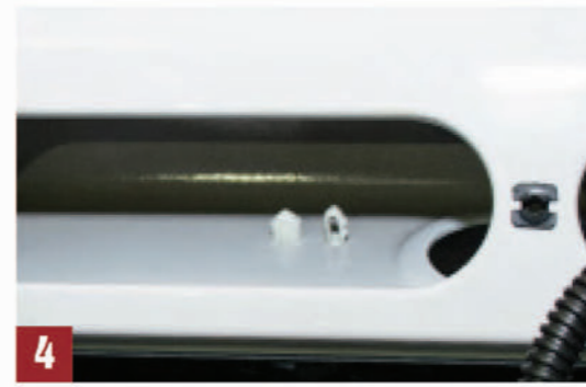
Fig. 2-3 Using a 9/32"(7mm) nut driver, remove the four (4) screws holding the housing in place and pull away from the cab. Fig. 4-7 Disconnect the light housing at the pigtail connector - not at the light. Access the connector by pushing down on the clips and pulling through the opening on the right. Disconnect by pressing down on the retaining clip, then slide away from each other. Place the removed housing in a safe location to be re-installed later.
