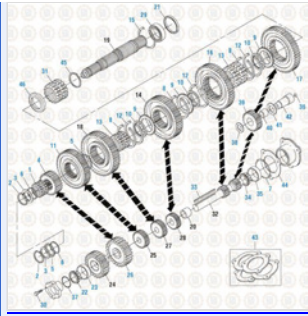
Drive Train 2016 Main Case Components - T2060A
