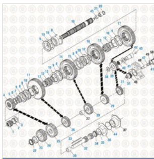
Drive Train 2016 Main Case Components - T2080B
