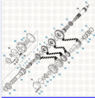
Web Electronic Main Case Components - Mack Transmission
