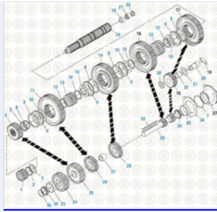
Drive Train 2016 Main Case Components - T309L and T310
