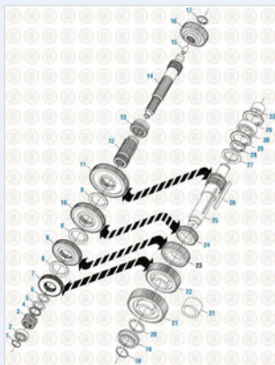
Drive Train 2016 Main Case Components - TRTXL-107/1070
