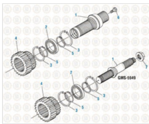
Drive Train 2016 Auxiliary Mainshaft Update - T2130 and T2180
