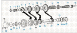
Web Electronic Main Case Components - Mack Transmission
