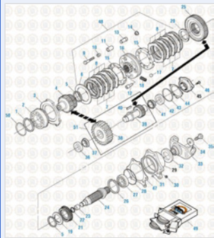
Drive Train 2016 Rear Case Components - Original Design Synchronizer - T2080, T2090 and T2100
