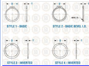
Hardware External - Basic and Inverted
