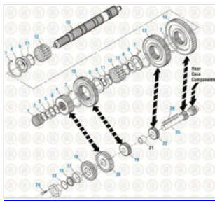
Drive Train 2016 Main Case Components - Long Rear Case, Multi-Speed Reverse, Rear Mounted Main Shifter - T2070 B & D
