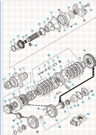
Drive Train 2016 Rear Case Components - T2080B
