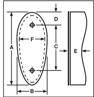
Pad Dimensions
