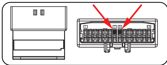
FIG A. (28 pin RP4.2 connector)
