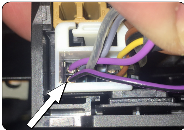
Picture of wire in 2014 - 2016 vehicle
