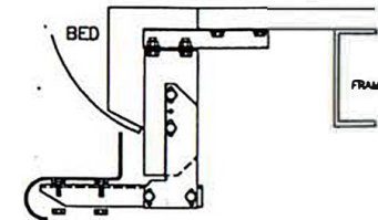
6 1/2' BED. REAR BRACKET
