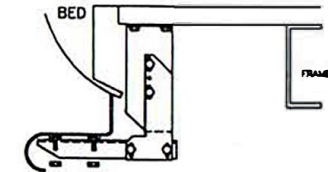
6 1/2' BED. REAR BRACKET
