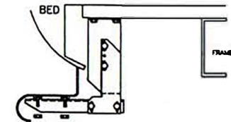
6 1/2' AND 8' BEDS. FRONT BRACKET
