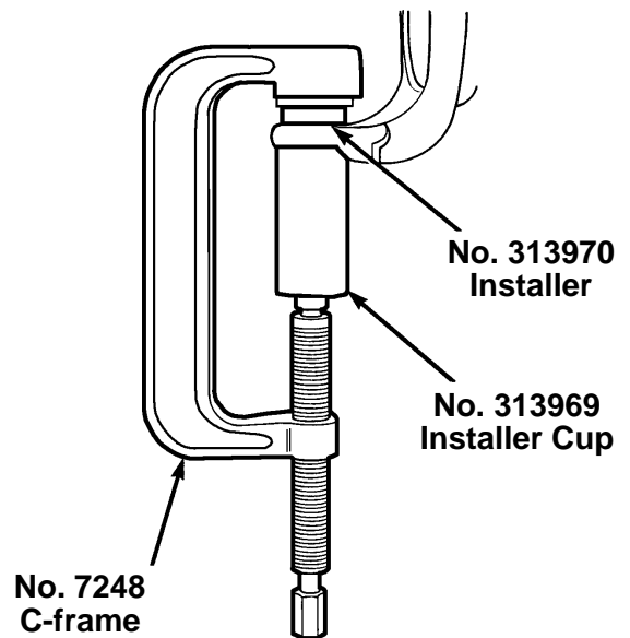
Installing the Lower Ball Joint
