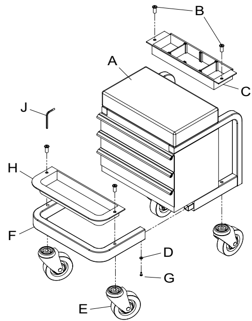
Figure 2 - 92450 Parts Breakdown
