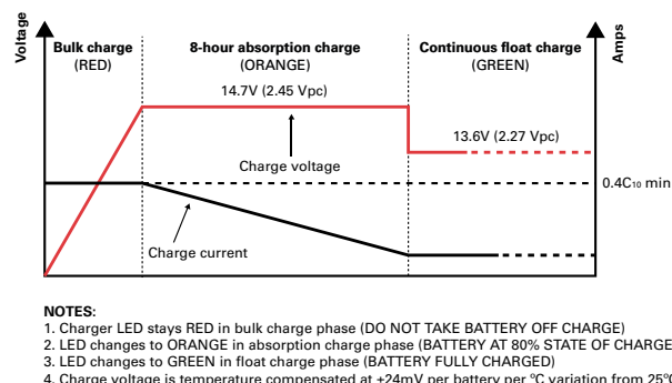
Figure 6: Recommended three-step charge profile
