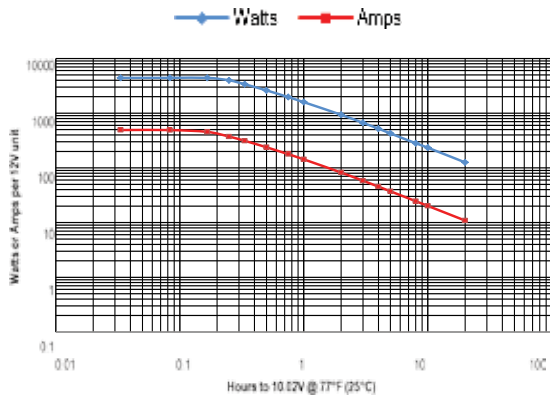
PC1800-FT performance data at 77°F, per 12V module
