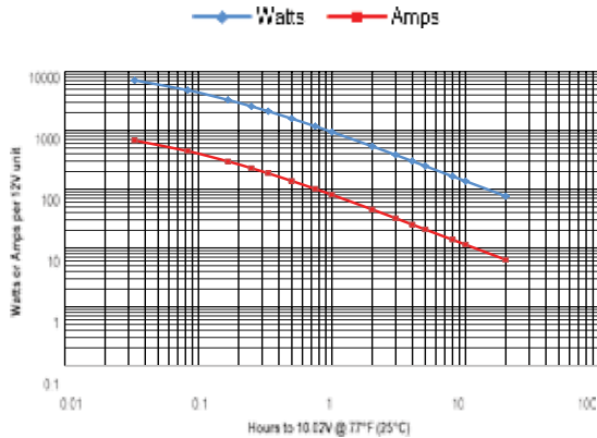
PC2250 performance data at 77°F, per 12V module
