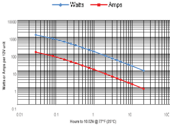
PC680 performance data at 77°F, per 12V module
