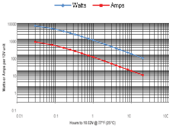
31-PC2150 and 31M-PC2150 performance data at 77°F, per 12V module
