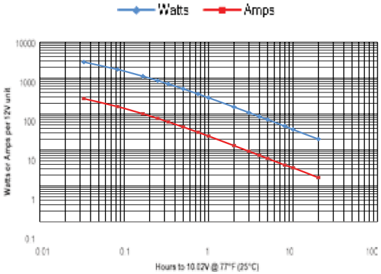
PC950 performance data at 77°F, per 12V module
