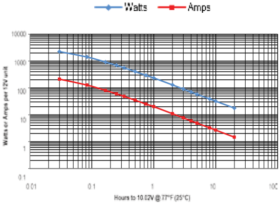
PC925 performance data at 77°F, per 12V module
